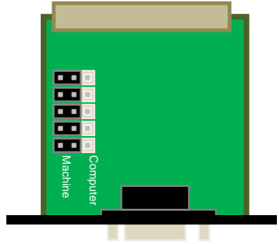
MCS-RS422 Interface In “To Machine” Configuration
