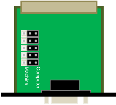
MCS-RS422 Interface In “To Computer” configuration
